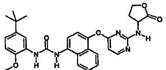
1-(5-tert-Butyl-2-methoxy-phenyl)-3-{4-[2-(2-oxo-tetrahydrofuran-3-ylamino)-pyrimidin-4-yloxy]-naphthalen-1-yl}-urea;
